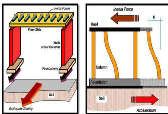
Fig. 1- Effect of Inertia in a building when shaken at its base
