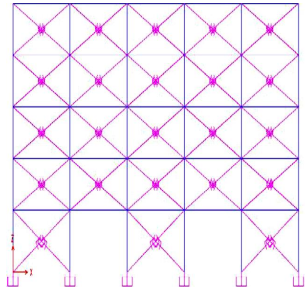
(b) Tension only cross braced friction dampers
