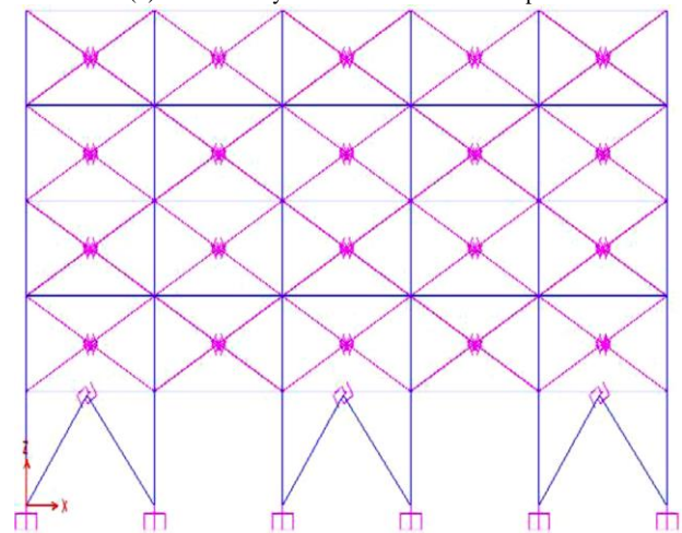
(c) Chevron braced friction damper
