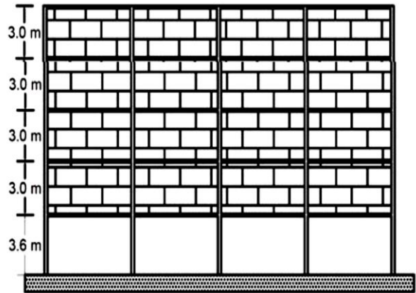
Fig. 5- Elevation of the prototype building. G+4 storey
