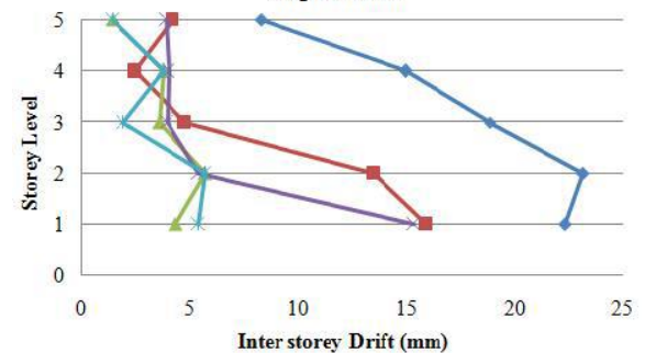
Fig. 8- Inter storey drift of building with and without dampers for the considered ground motions
