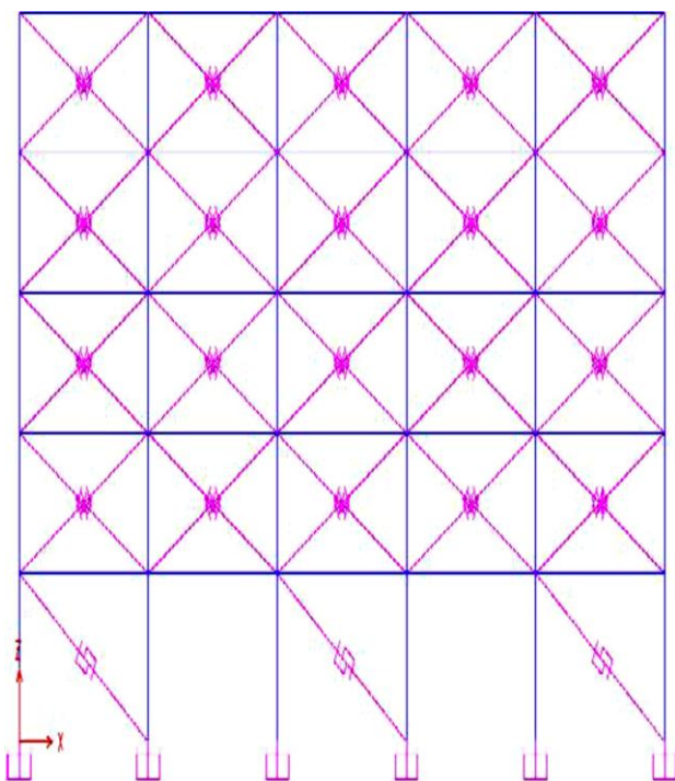
(a) Single diagonal tension/compression friction damped bracing
