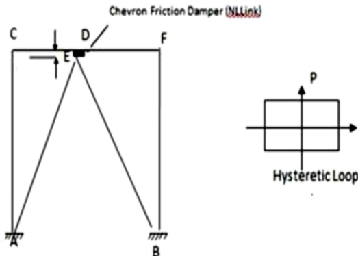
Fig. 3- Chevron Brace with Pall Friction Damper
