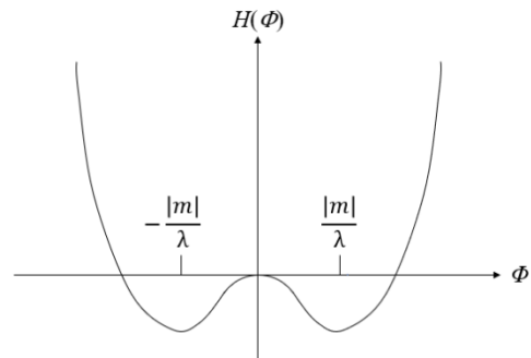
Figure 6. Two local minimums in the Higgs potential of the scalar field \Phi .
