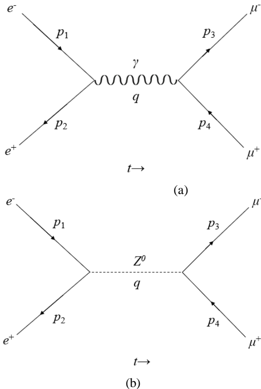
Figure 3. (a) The Feynman diagram about the electromagnetic contribution to e^+ + e^- \rightarrow \mu^+ + \mu^- . (b) The Feynman diagram about the weak contribution to e^+ + e^- \rightarrow \mu^+ + \mu^- .
