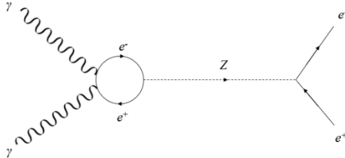
Figure 2. The possible Feynman diagram for two photons through the electronbubble and Z boson intermediates to become to an electron-positron pair.
