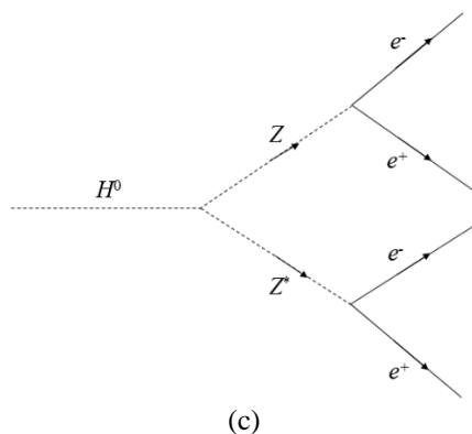
Figure 4. (a) The fundamental vertex of direct coupling between the electron and Higgs boson. (b) The Feynman diagram of the interaction between two electrons through the intermediate Higgs boson. (c) The Feynman diagram for the process decaying from the Higgs field to the final four leptons such as electrons [7].
