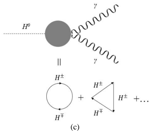
Figure 1. (a) The electron-positron pair production describing in QED. (b) Two-photon production by the electron-positron pair annihilation also describing in QED. The other diagram can be drawn by interchanging two outgoing photons. (c) The neutral Higgs boson decays to two photons including the parts of vertices [8,9].
