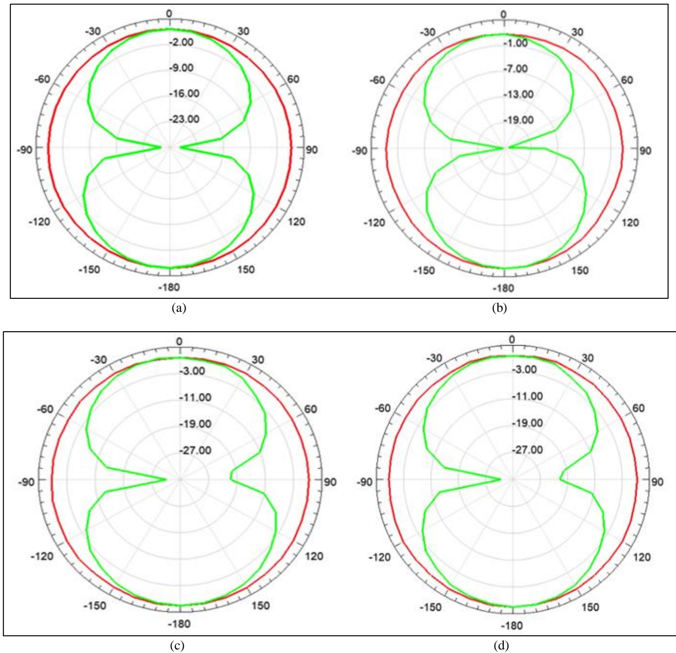
Fig 4:- Radiation pattern of (a) Two-dimensional microstrip patch antenna, (b) Conformal MPA with R1=15mm, (c) Conformal MPA with R2=30mm, (d) Conformal MPA with R3=45mm
