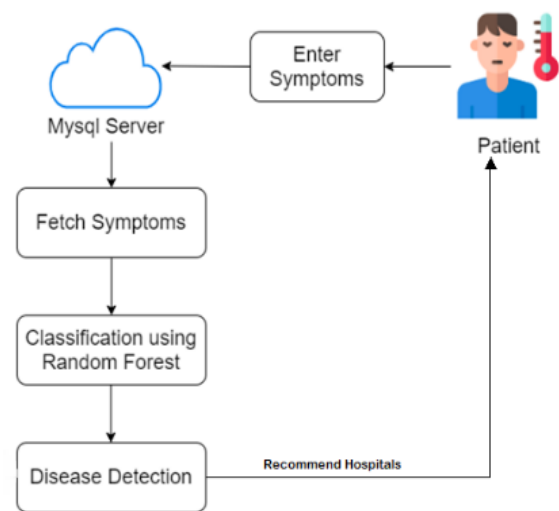
Fig. 1: System Architecture
