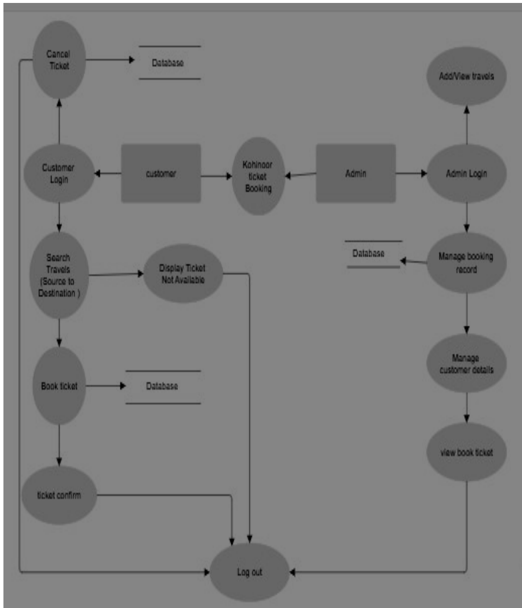
Fig 1 DFD 2 Diagram
