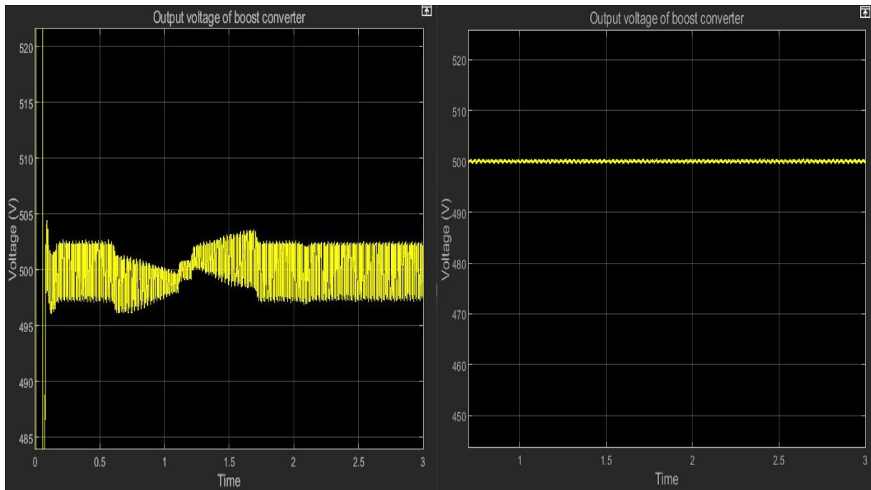
Fig. 19: A comparison of output voltage of boost converter in both cases
