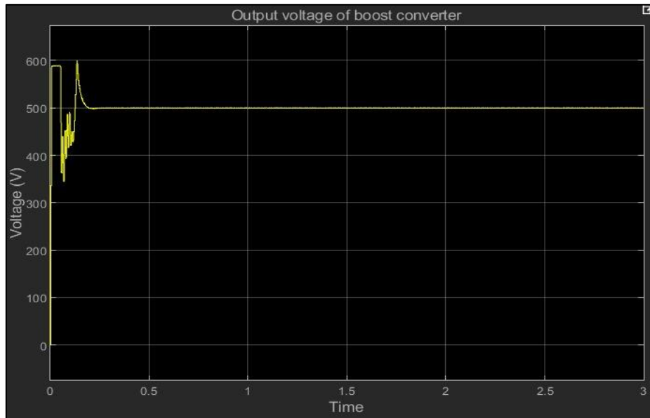
Fig. 17: Output voltage of boost converter controlled by FLC
