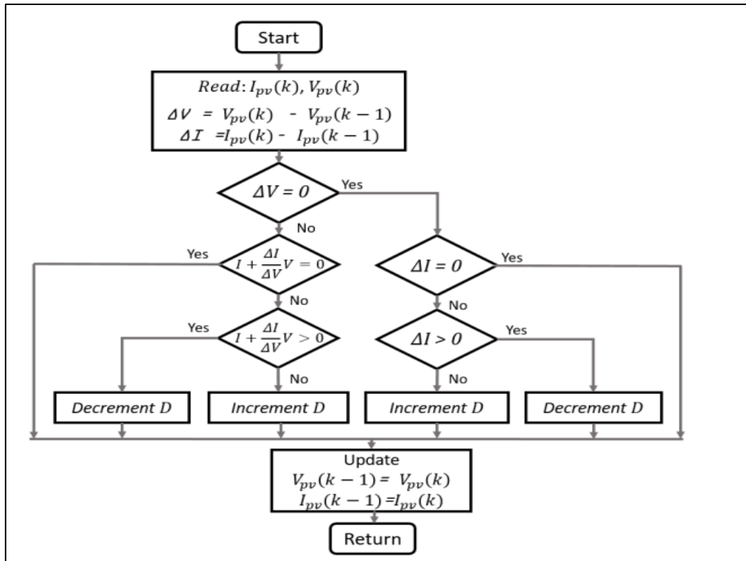
Fig. 7: Incremental conductance chart
