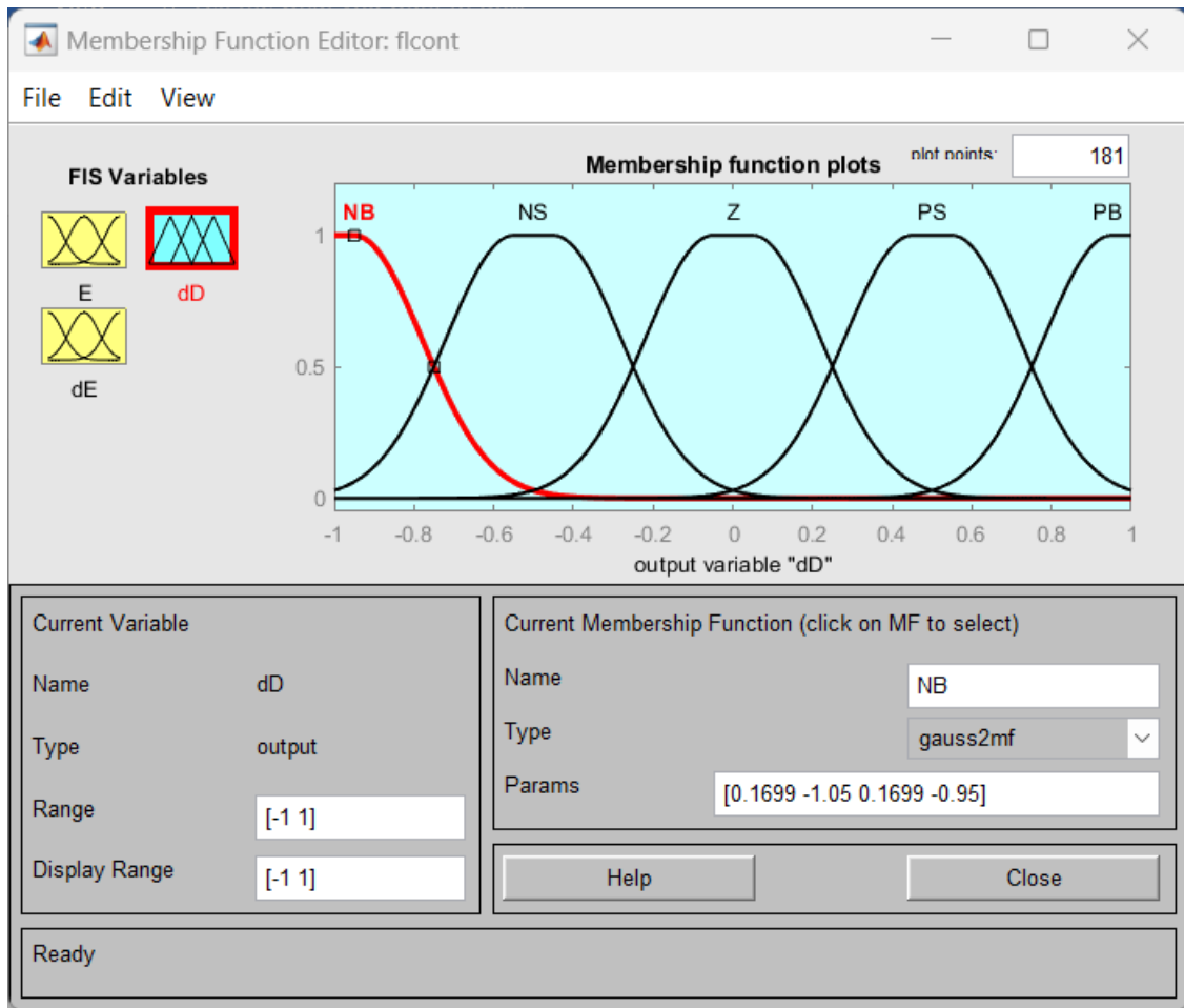
Fig. 13: Membership functions of Output.
