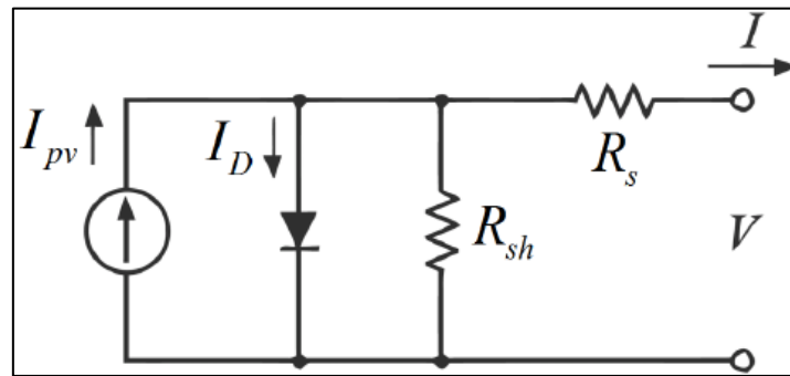
Fig. 3: Photovoltaic cell equivalent circuit.
