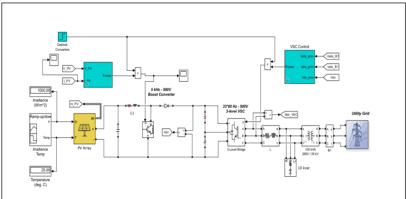
Fig. 2: Grid-Connected PV Array with MPPT controller
