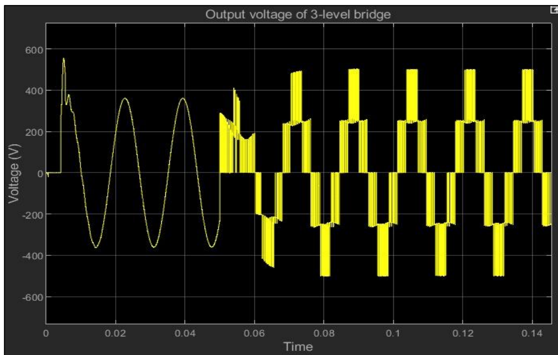
Fig. 16: three-level bridge voltage
