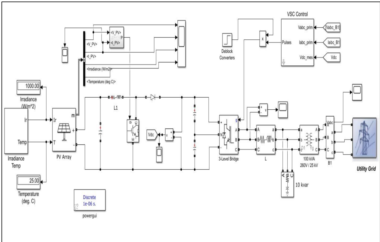
Fig. 8: Grid-Connected PV Array with fuzzy logic controller
