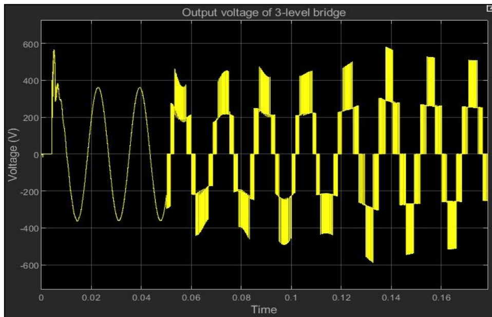
Fig. 18: three-level bridge voltage
