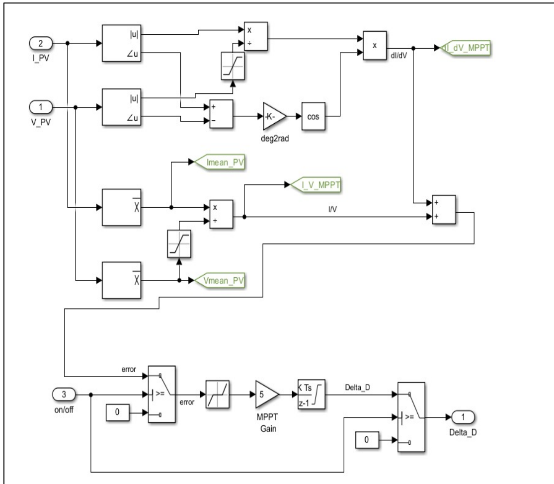
Fig. 6: Incremental Conductance Method blocks
