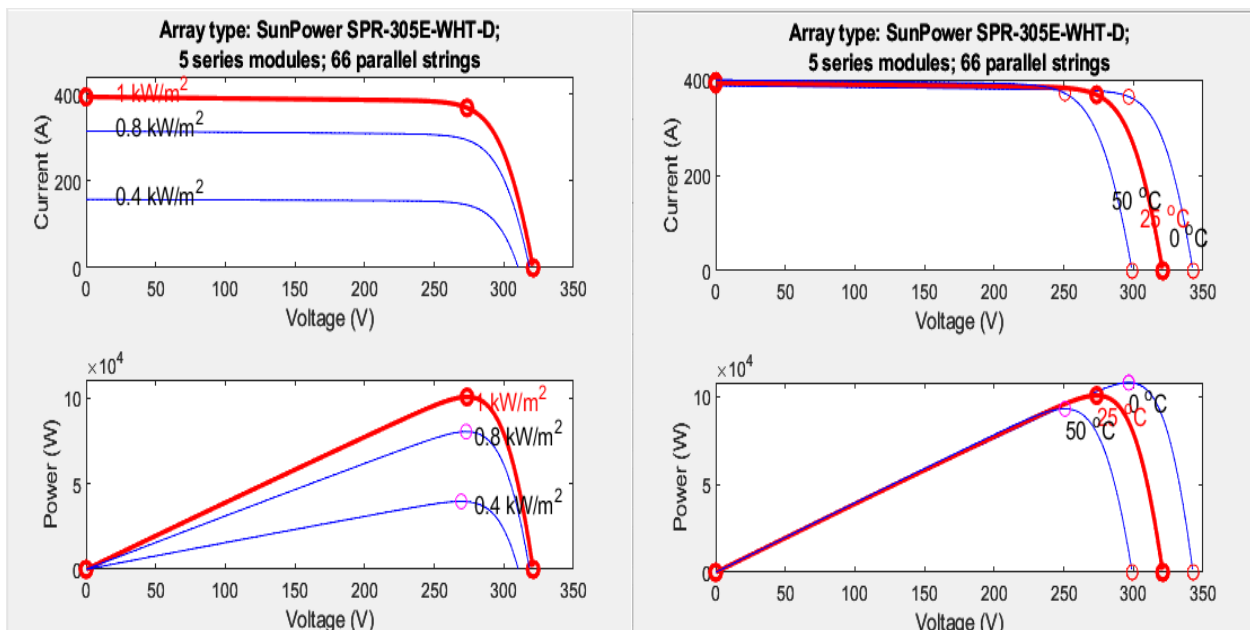
Fig. 4: IV curve under environment variations
