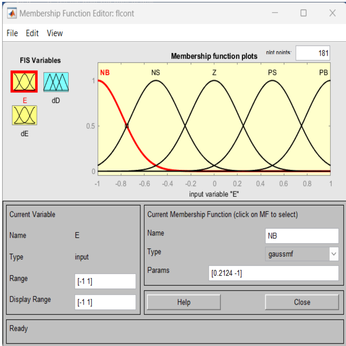
Fig. 12: Membership functions of Inputs
