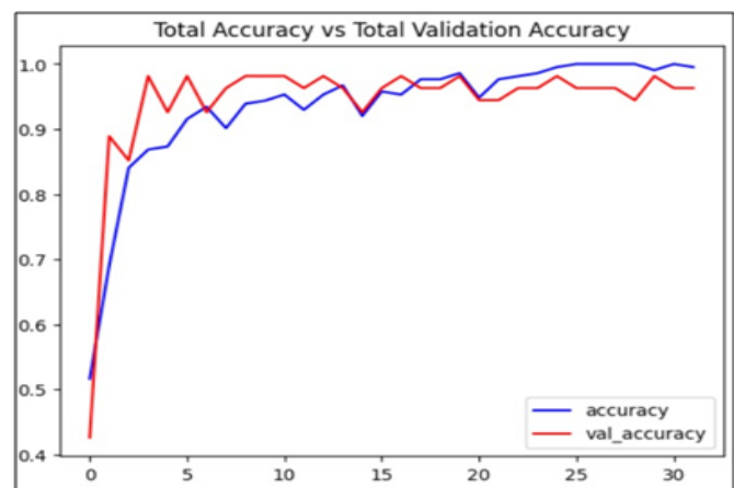
Fig 4 Accuracy Graph
