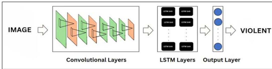
Fig 1 Conv -LSTM Network's Structure
