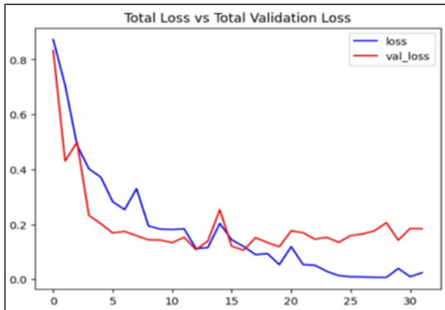
Fig 5 Loss Graph
