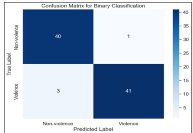
Fig 3 Confusion Matrix
