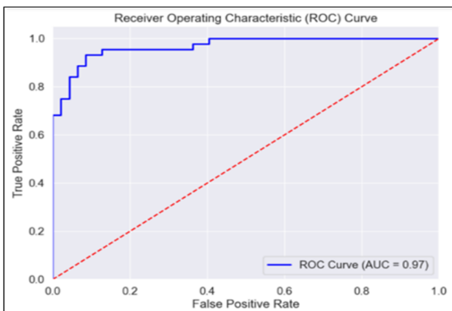
Fig 6 Roc Curve
