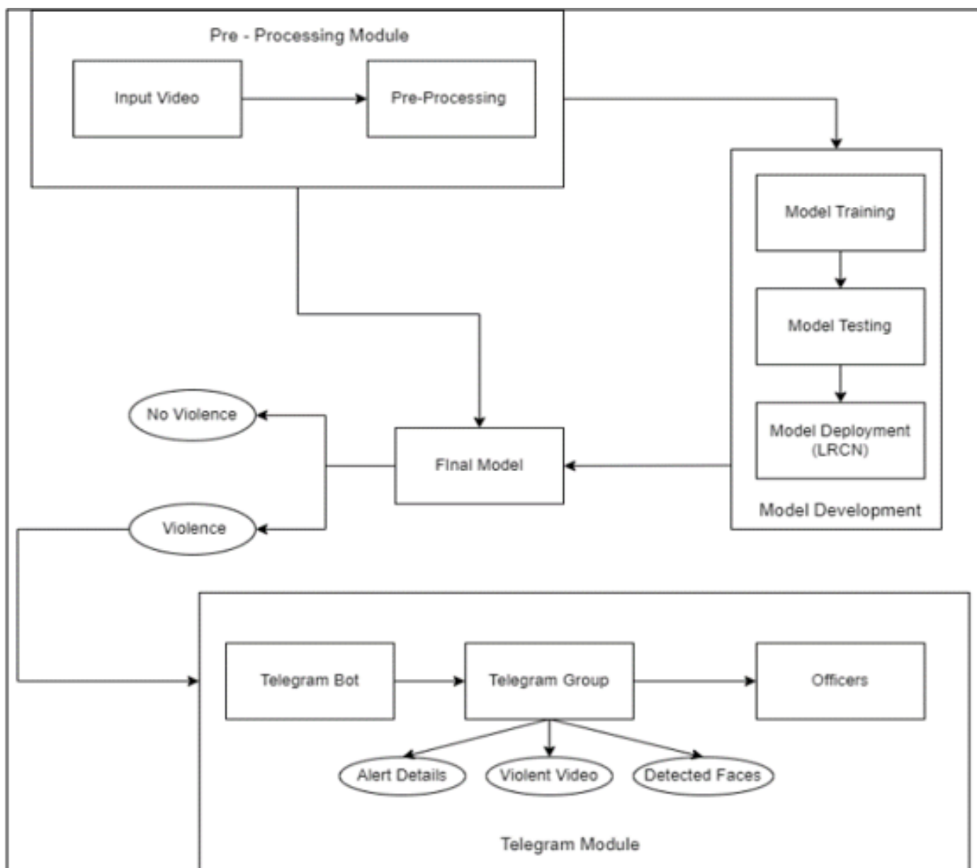
Fig 2 Architecture of Violence Detection Model
