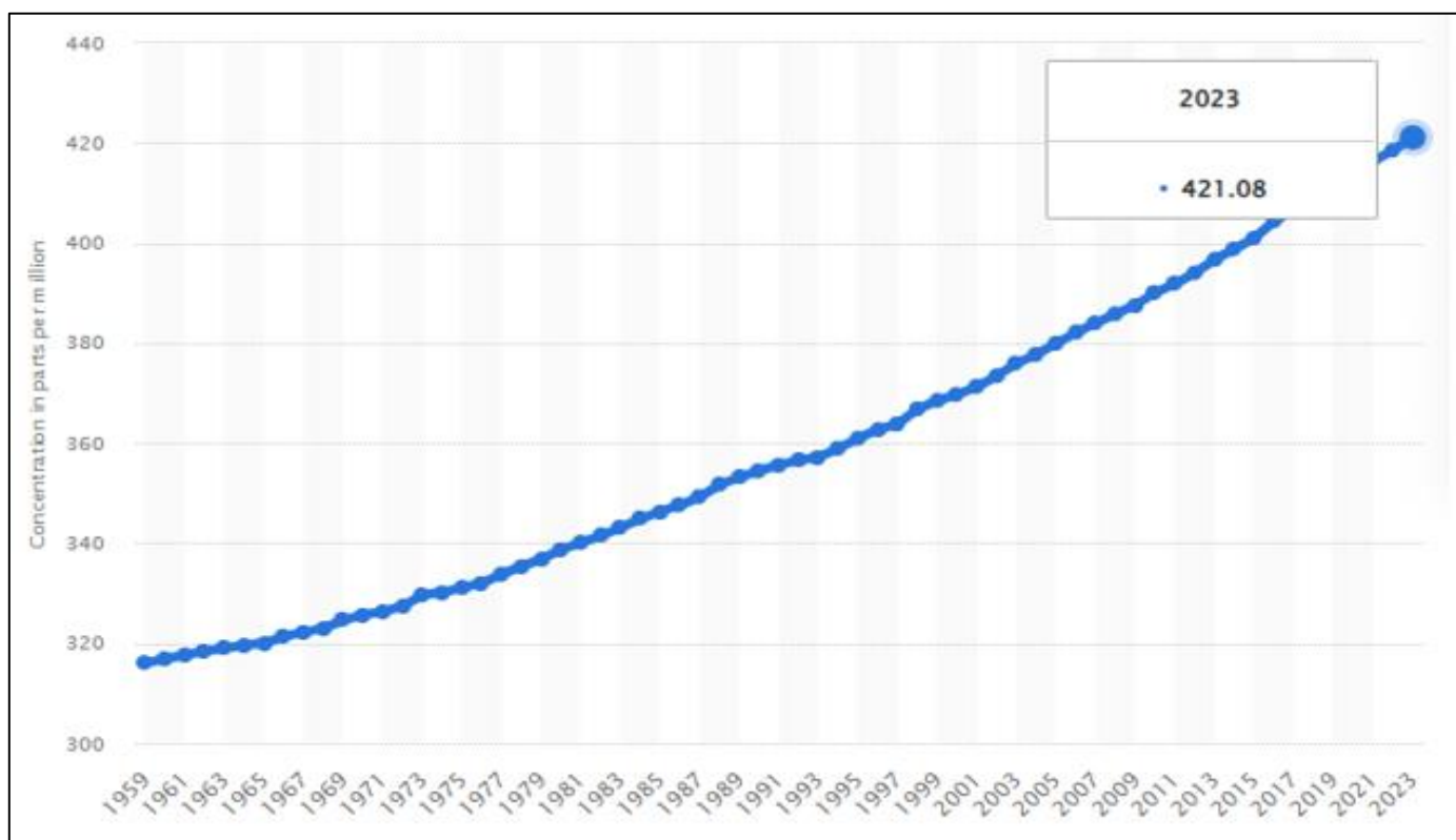
Fig 1: Direct measurement of atmospheric CO 2 from 1959 to 2023 in ppm
