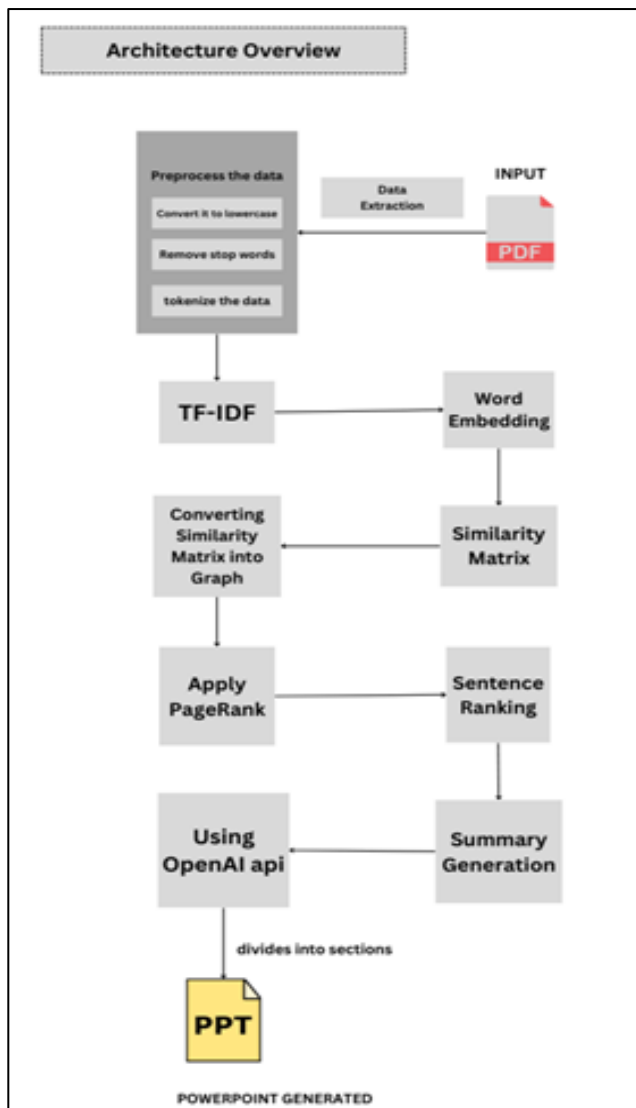
Fig. 1. Architecture of Proposed System
