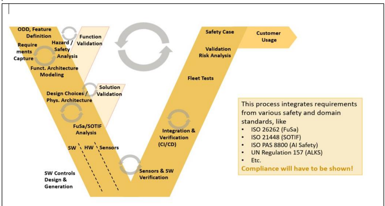
Fig 6 Agile MBSE methodology integrating safety and validation activities [22]
