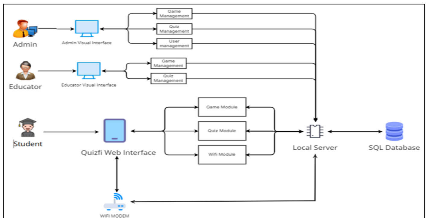
Fig 1 The Diagram Illustrates the QuizFi System, The QuizFi System Connects Administrators, Educators, and Students through Game, Quiz, and user Management Modules. It Runs on a Local Server with an SQL Database for Efficient Data Handling
