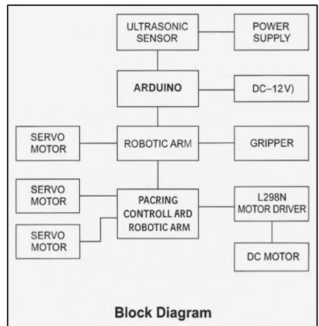
Fig 1 Block Diagram
