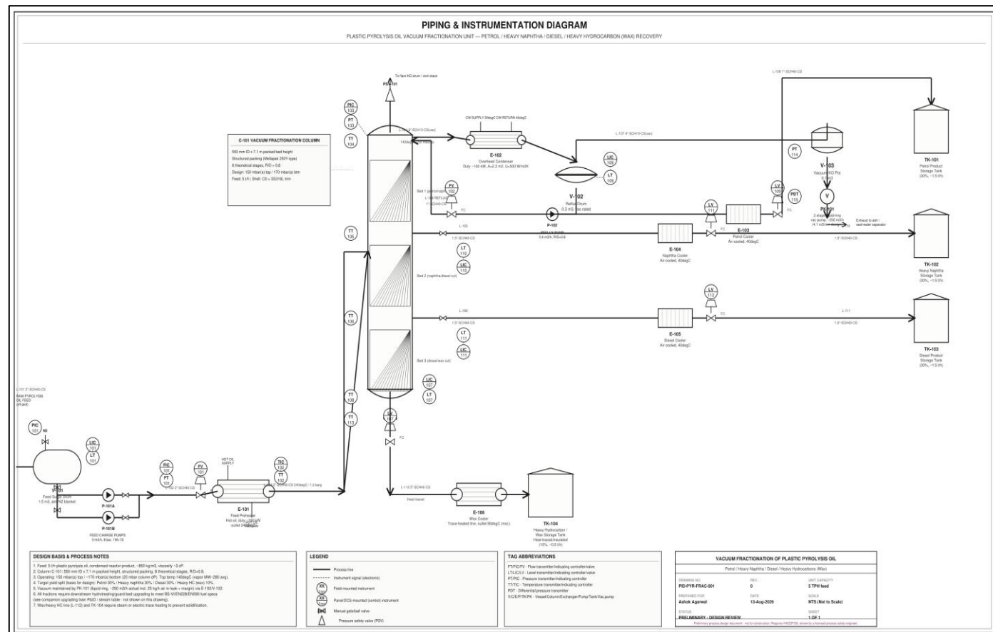
Fig 1 Conceptual Process Flow Diagram
