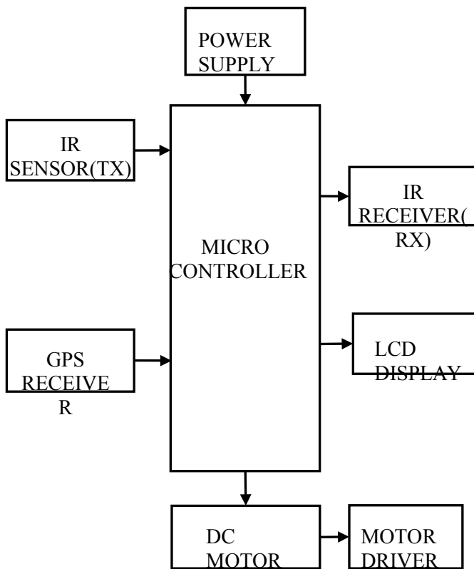
Fig 3.1 Block diagram of Railway track crack detection
