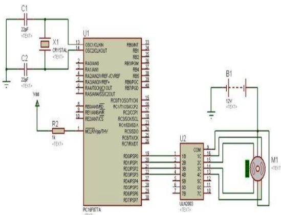
Fig 5:- Circuit Diagram of Motor Driver
