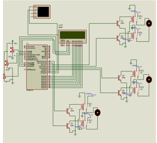
Fig 6:- Simulation in Proteus
