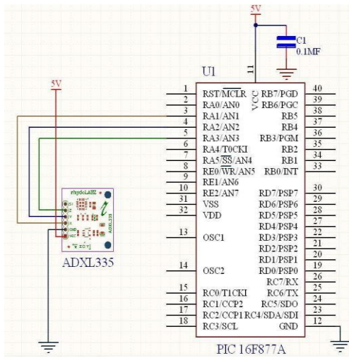
Fig 4:- Circuit Diagram of MEMS Sensor
