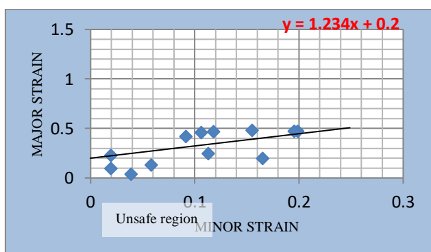
Graph 5. FLD for Cupping test with Wall angle of 40°
