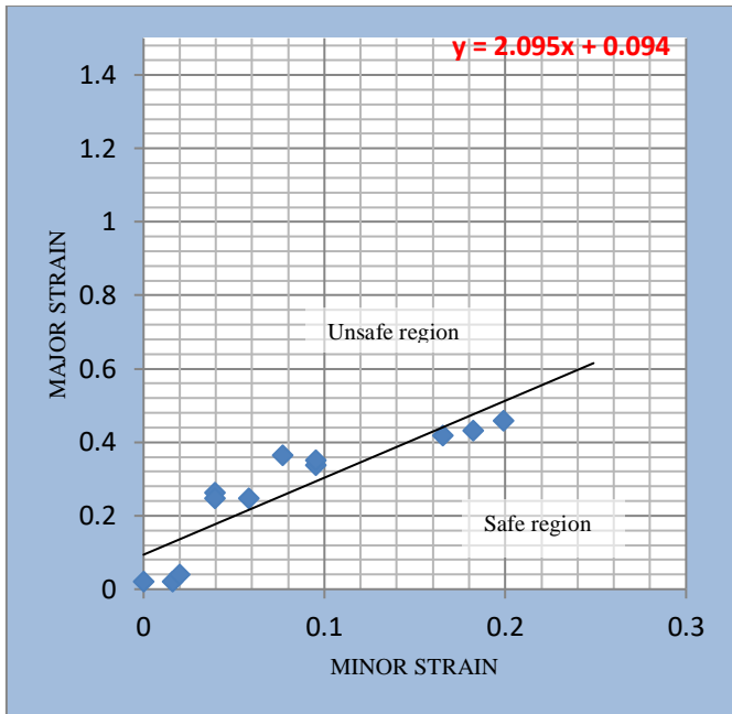
Graph 6. FLD for Cupping test with Wall angle of 45°
