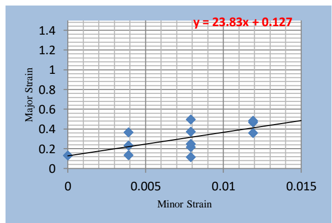
Graph 1. FLD for Straight groove length of 40mm
