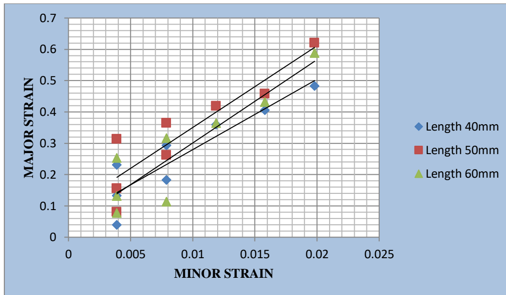
Graph 4. Combined FLD for Straight Groove Length of 40mm, 50mm and 60mm.
