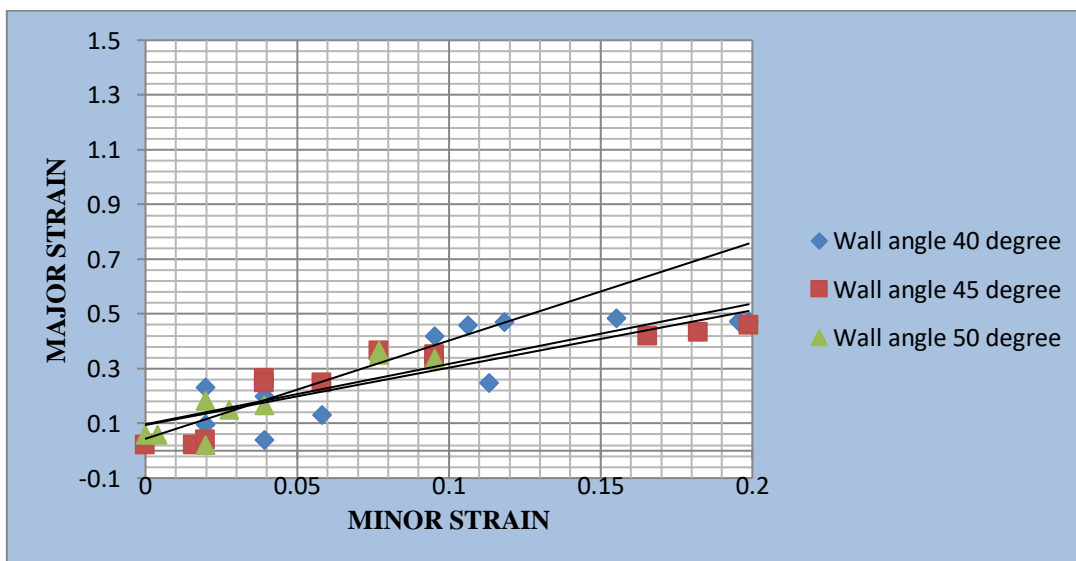
Graph 8. Combines FLD for Cupping test with Wall angle of 40°, 45° and 50°.
