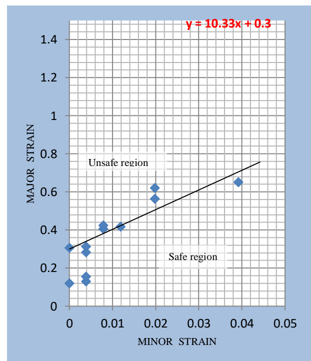
Graph 3. FLD for Straight groove length of 60mm
