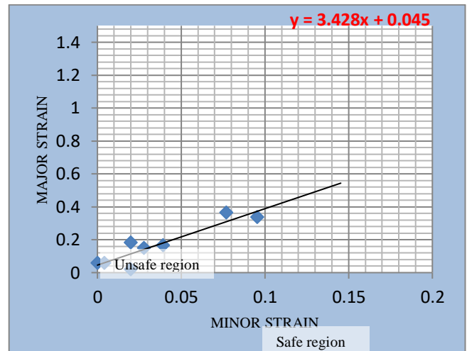
Graph 7. FLD for Cupping test with Wall angle of 50°
