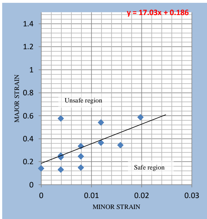
Graph 2. FLD for Straight groove length of 50mm
