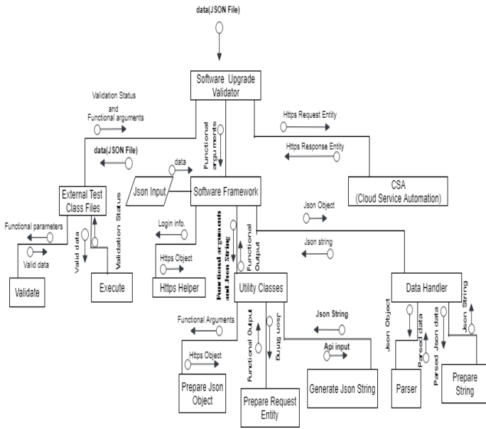
Fig 4:- Structure Chart of proposed Framework
