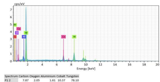
Fig 4:- EDX analysis for PVD tool insert
