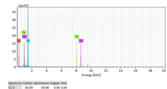
Fig 5:- EDX analysis for CVD tool insert
