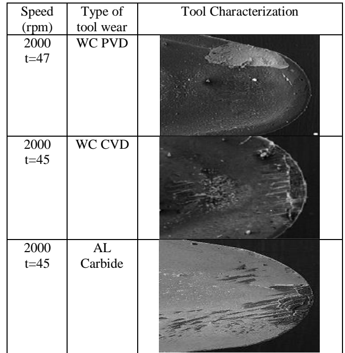
Fig 3:- Optical micrographs of surface roughness on different cutting tools after machining AA7075 alloy at giving better surface roughness speed and machining time
