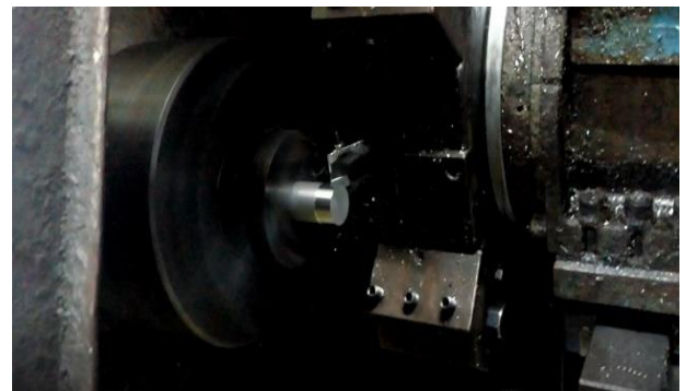
Fig 2:- CNC turning of AA7075
