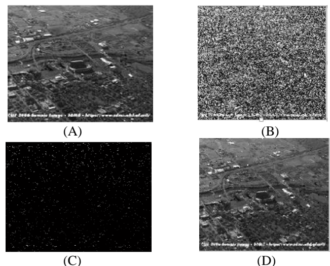
Fig 4:- (A) Depicts the Original SAR Image, (B) Depicts the Image after N Oise is Added, (C) Depicts the Image after Pre-Processing, (D) Depicts the Filtered SAR Image.
