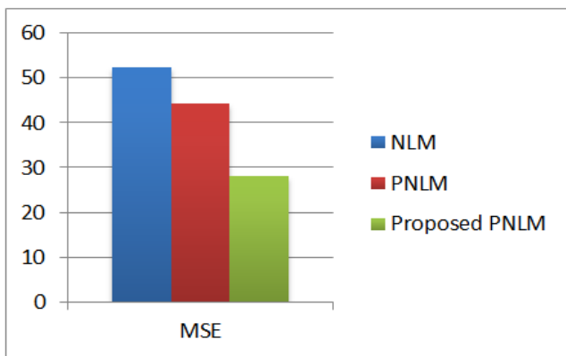
Fig 3:- MSE Comparisons
