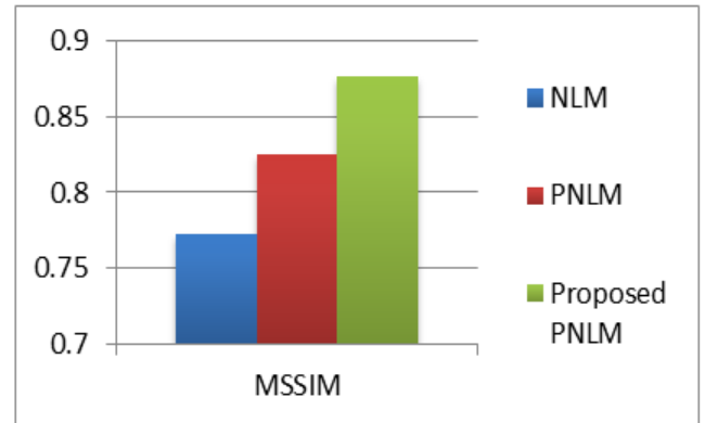
Fig 4:- MSSIM Comparison
