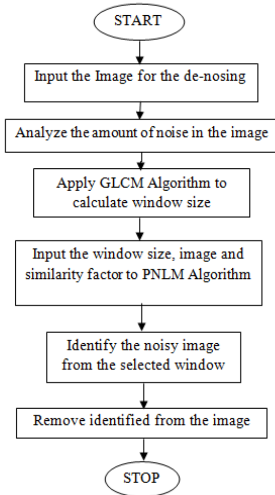
Fig 1:- Proposed Flowchart
