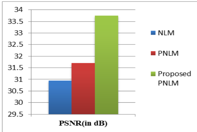
Fig 2:- PSNR Comparison
